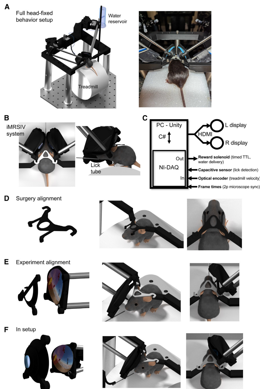
Figure 3. iMRSIV behavior apparatus and device-eye alignment procedures
