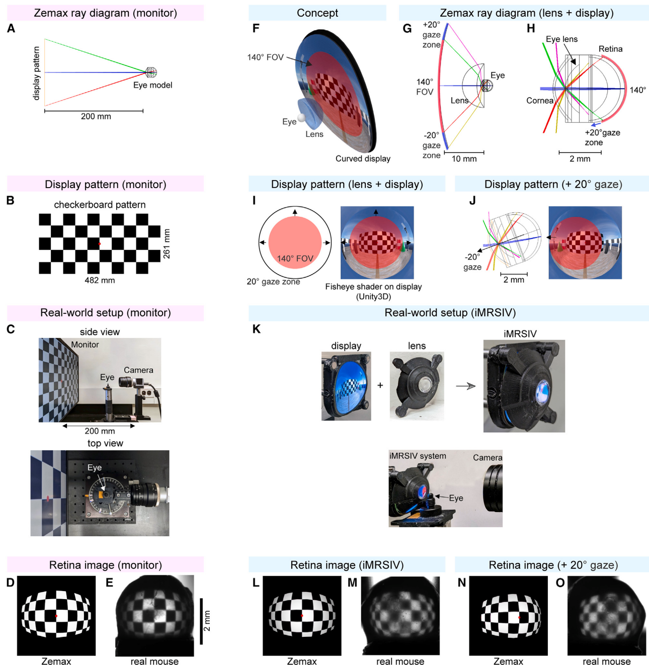
Figure 2. iMRSIV goggle device design and validation
